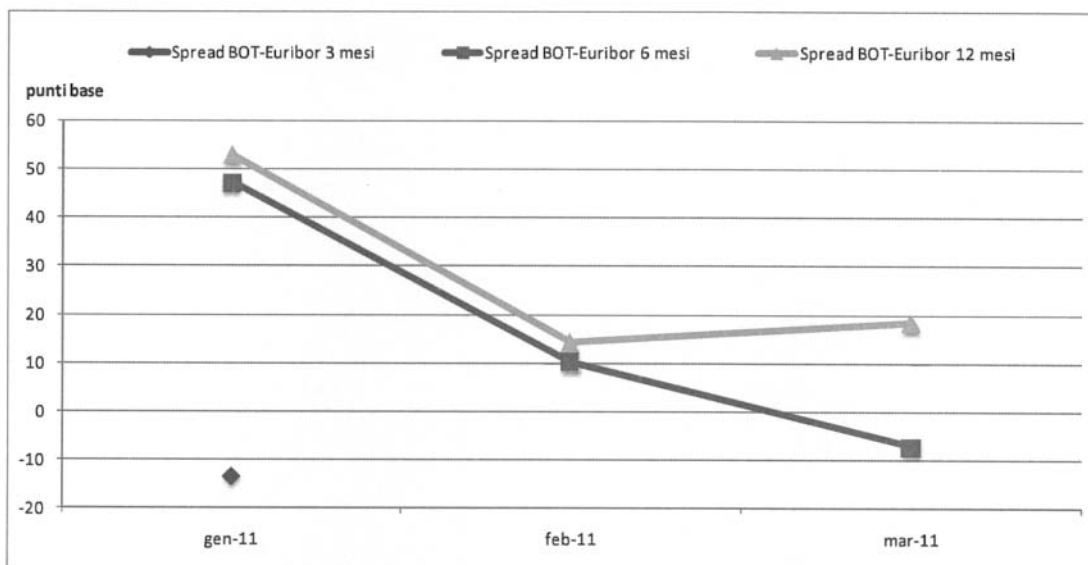
Figura 3-11: Spread Bot-Euribor.
