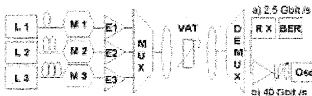
Fig. 17: Set-up sperimentale
